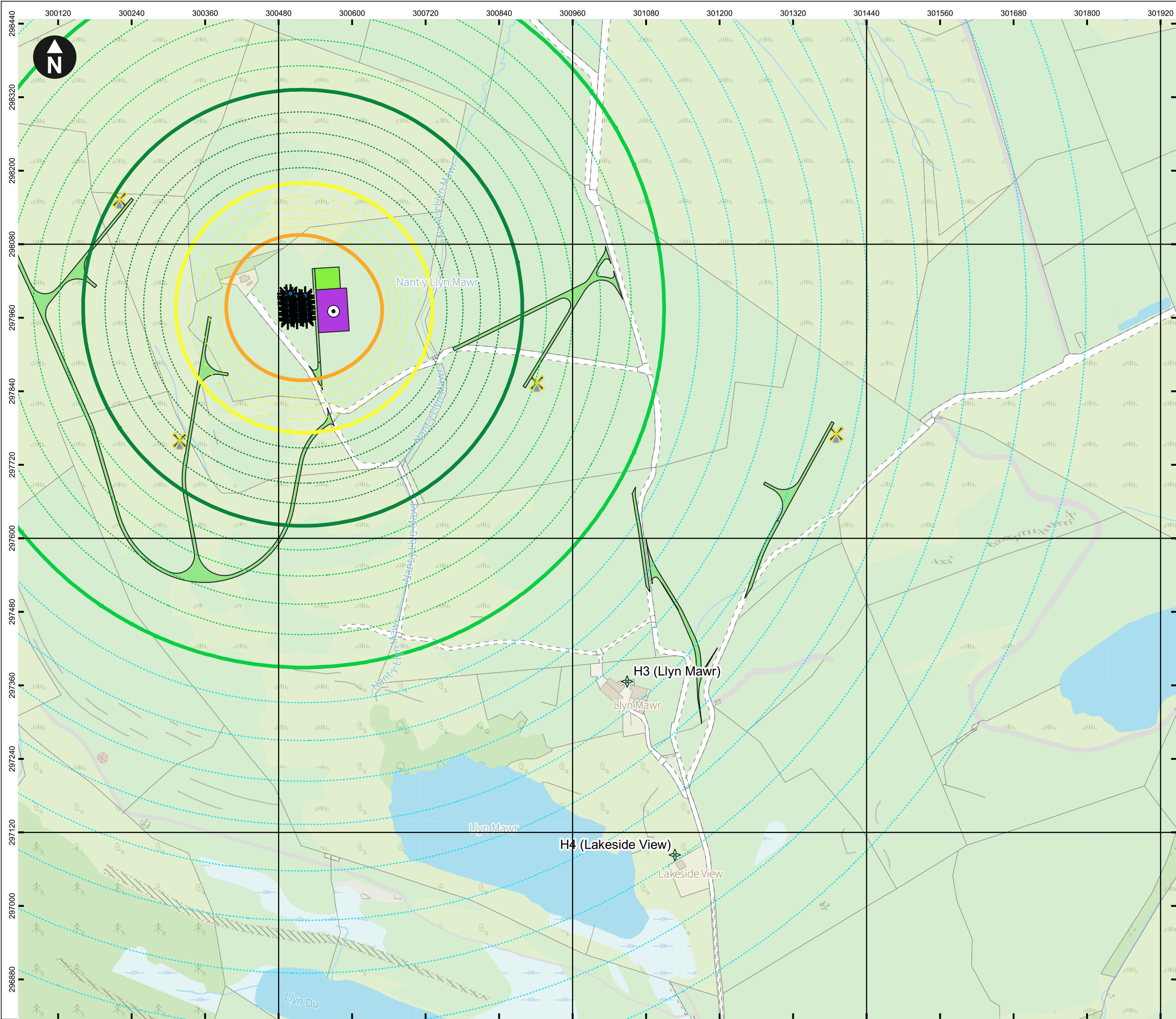
Figure 11.4 Predicted Operational BESS Noise Levels
