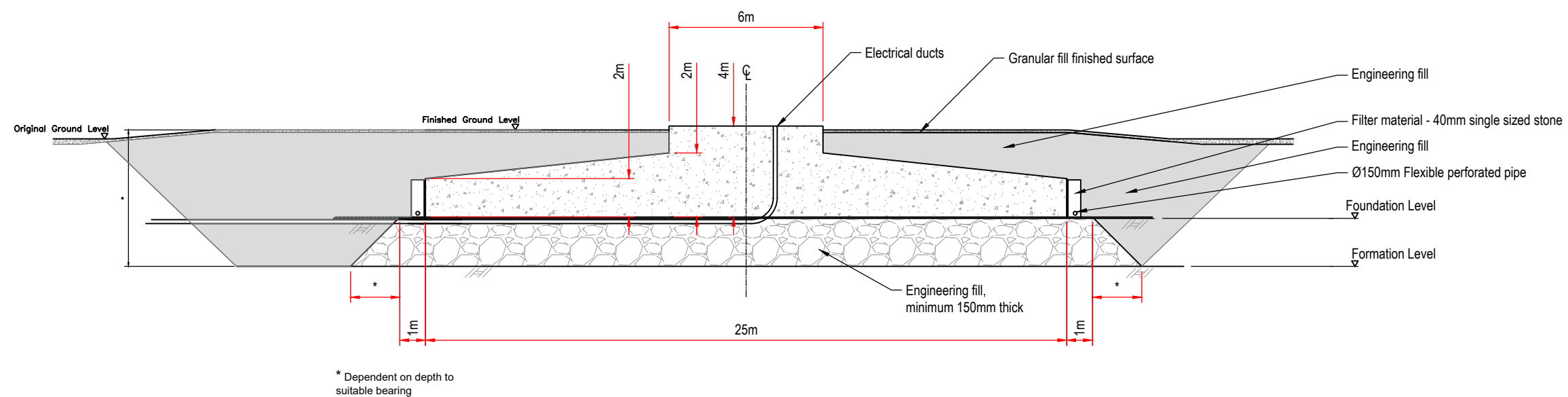
View on A-A'
