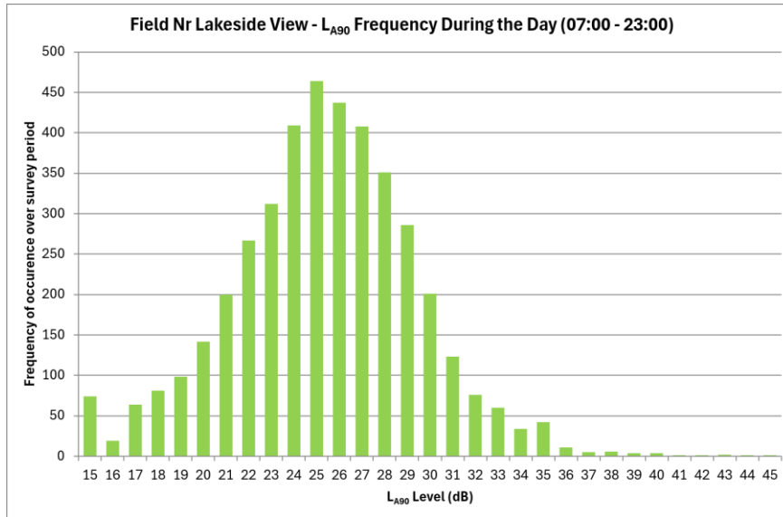
Plate 11D-84 - Field nr Lakeside View - L_{A90} Frequency During the Day
