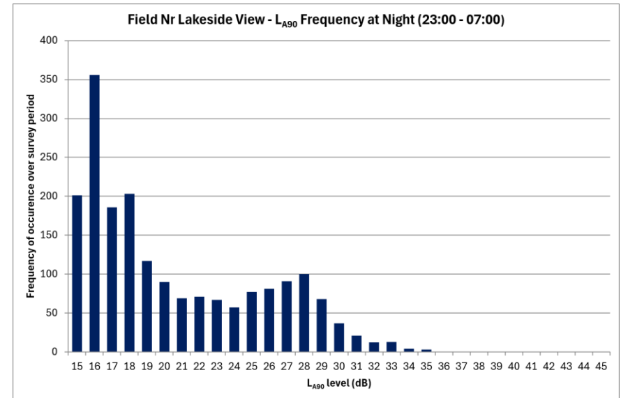
Plate 11D-85 - Field nr Lakeside View - L_{A90} Frequency During the Night
