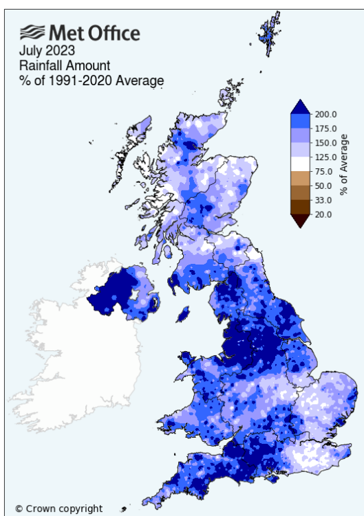
Plate 11I.24 – Rainfall amount (as percentage of 1991-2020 Average) – July 2023
