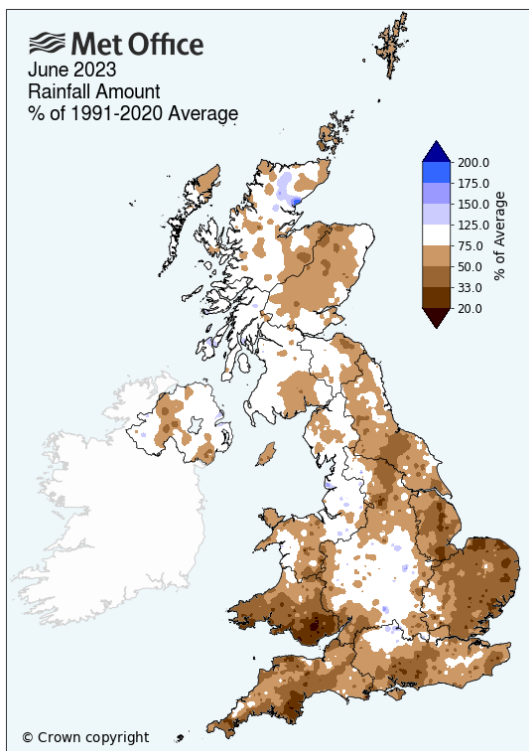
Plate 11I.23 – Rainfall amount (as percentage of 1991-2020 Average) – June 2023
