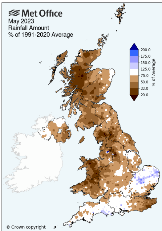
Plate 11I.22 – Rainfall amount (as percentage of 1991-2020 Average) – May 2023
