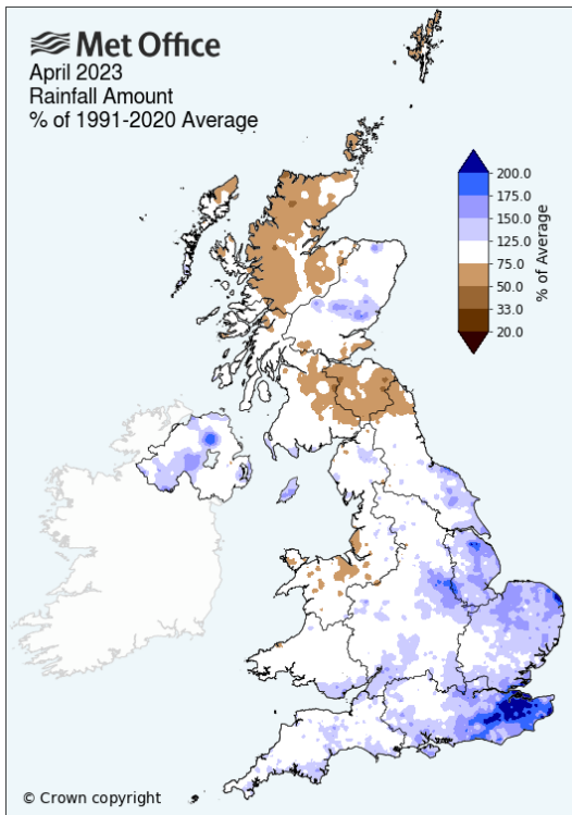
Plate 11I.21 – Rainfall amount (as percentage of 1991-2020 Average) – April 2023
